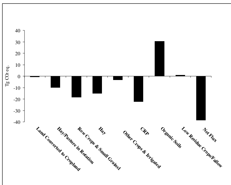
Figure 3-7. CO 2 Emissions and Sequestration from Cropland Soils, 2005
