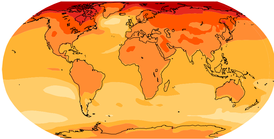
RCP8.5, 2046-2065 vs. 1986-2005
