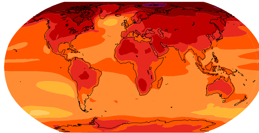
RCP8.5, 2081-2100 vs. 1986-2005
