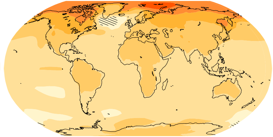
RCP2.6, 2081-2100 vs. 1986-2005
