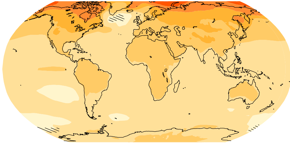
RCP8.5, 2046-2065 vs. 1986-2005
