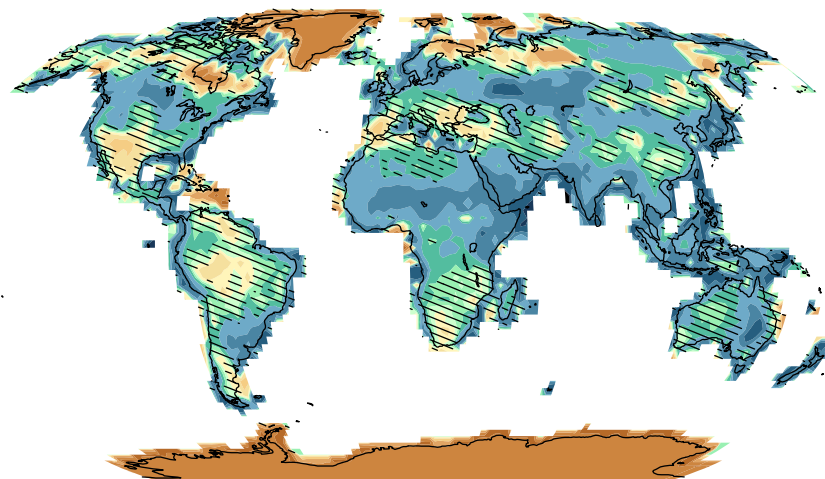
RCP8.5, 2046-2065 vs. 1986-2005
