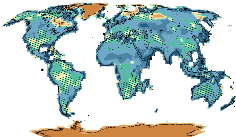
RCP2.6, 2046-2065 vs. 1986-2005
