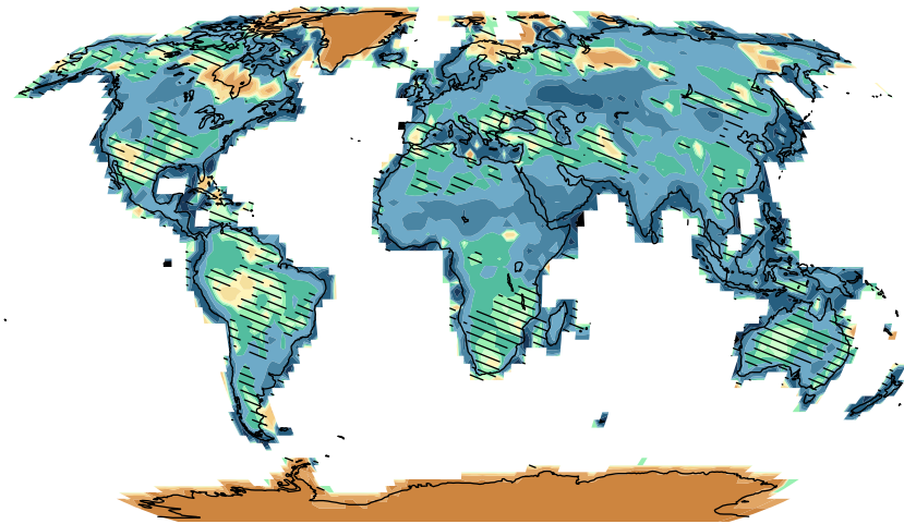
RCP2.6, 2081-2100 vs. 1986-2005
