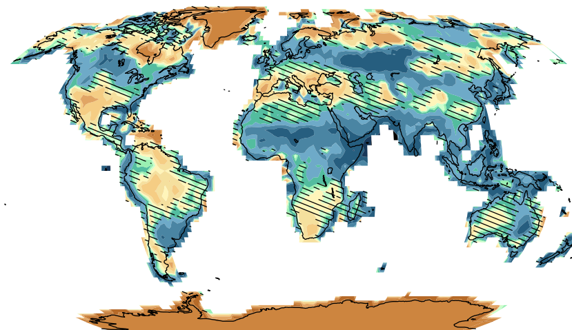
RCP8.5, 2081-2100 vs. 1986-2005
