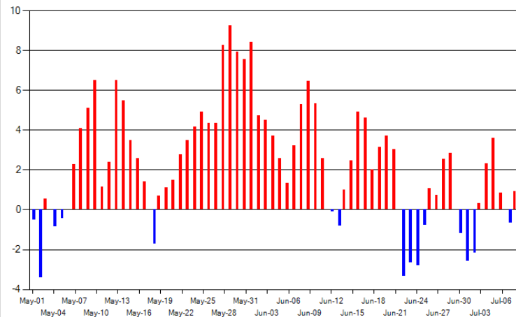
42 - NORTHEAST GERMANY Daily Temperature Departures From Normal May - Current
