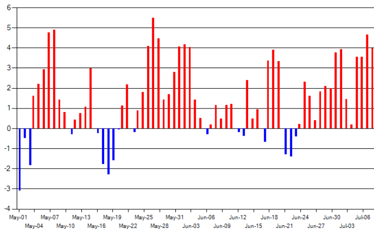
7 - SOUTHEAST ENGLAND Daily Temperature Departures From Normal May - Current
