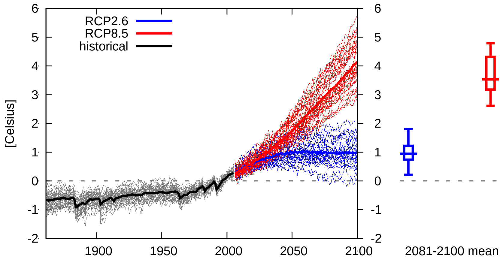
Temperature change World Jan-Dec wrt 1986-2005 full CMIP5 ensemble
