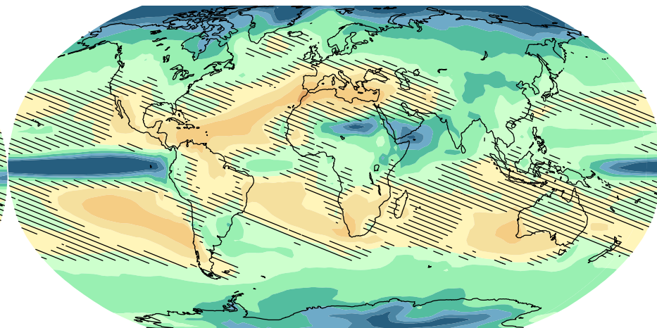
RCP8.5, 2081-2100 vs. 1986-2005
