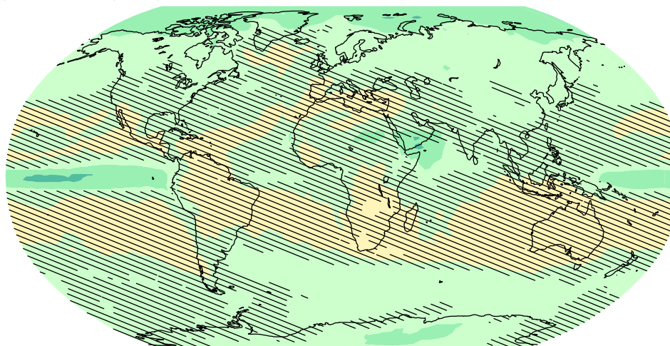
RCP8.5, 2081-2100 vs. 1986-2005
