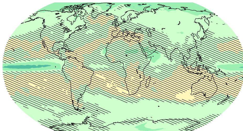
RCP8.5, 2046-2065 vs. 1986-2005
