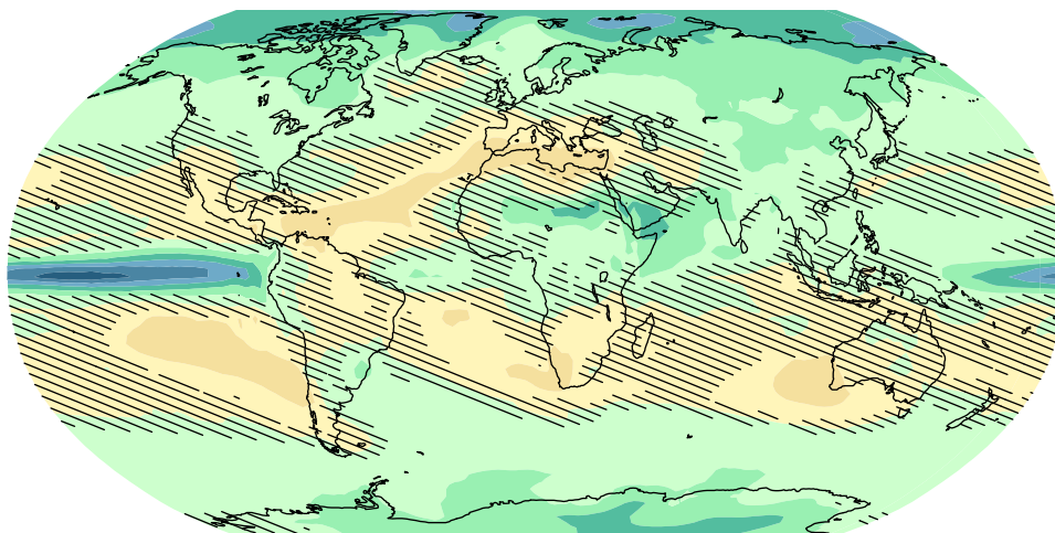
RCP8.5, 2046-2065 vs. 1986-2005
