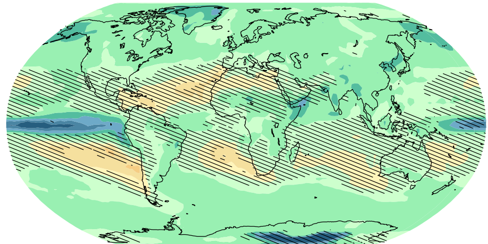
RCP8.5, 2081-2100 vs. 1986-2005
