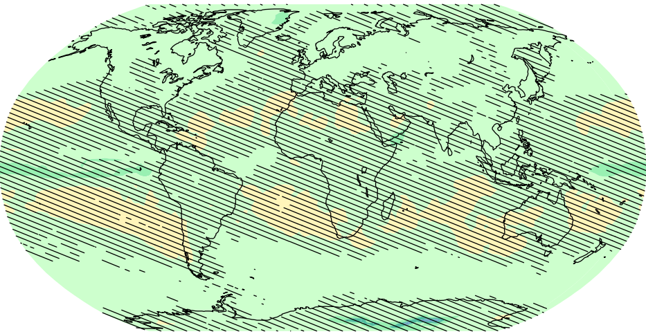
RCP2.6, 2046-2065 vs. 1986-2005
