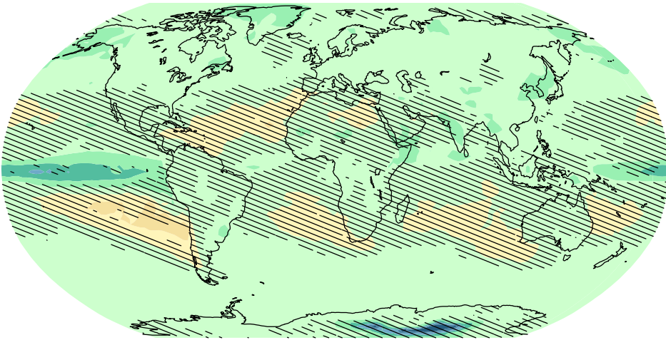
RCP8.5, 2046-2065 vs. 1986-2005
