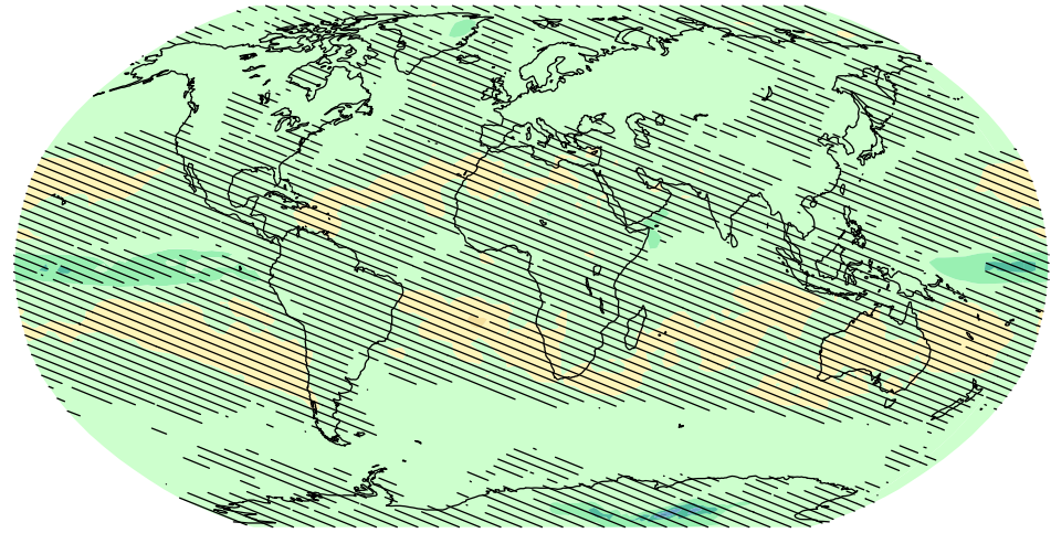
RCP2.6, 2081-2100 vs. 1986-2005
