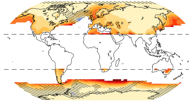
RCP2.6, 2081-2100 vs. 1986-2005
