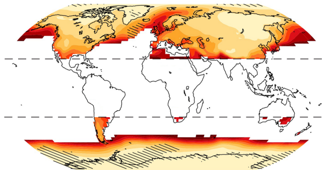
RCP8.5, 2046-2065 vs. 1986-2005
