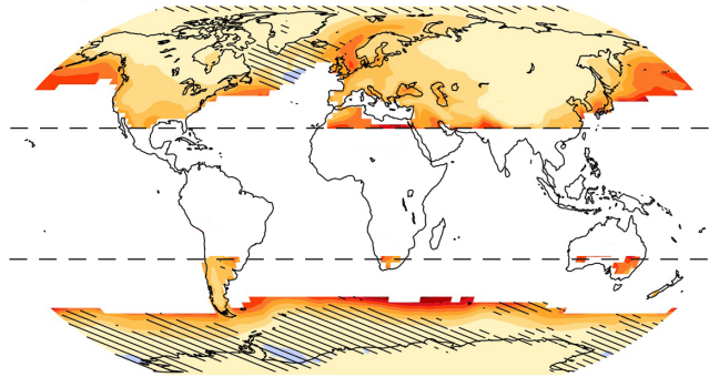
RCP2.6, 2046-2065 vs. 1986-2005
