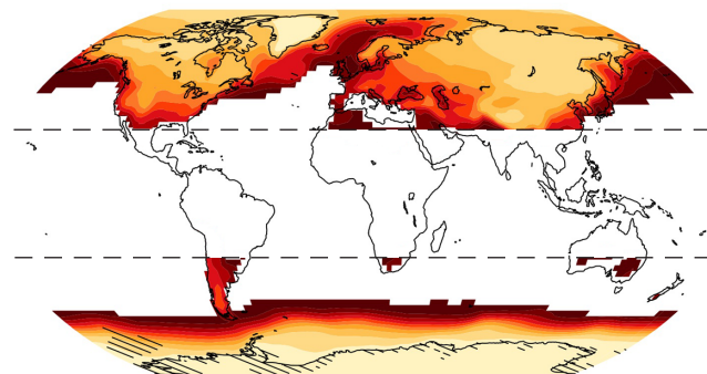
RCP8.5, 2081-2100 vs. 1986-2005
