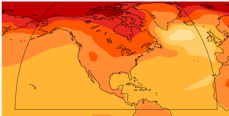
RCP8.5, 2046-2065 vs. 1986-2005
