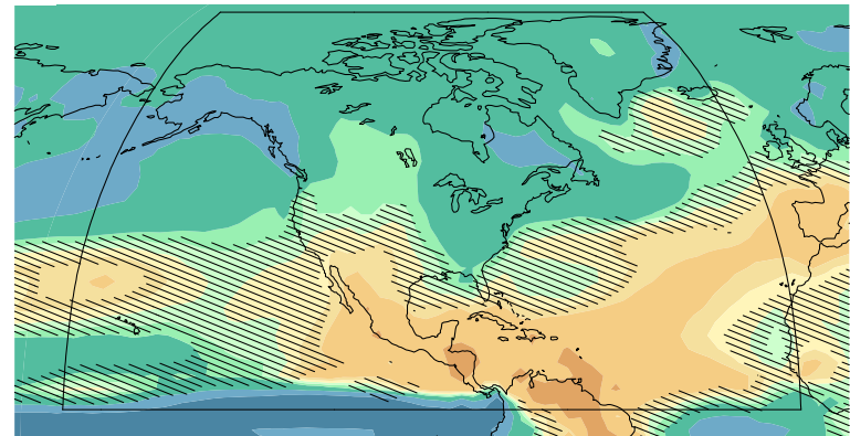
RCP8.5, 2081-2100 vs. 1986-2005
