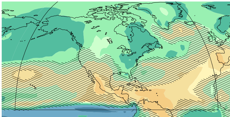
RCP8.5, 2046-2065 vs. 1986-2005
