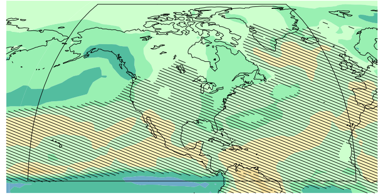
RCP2.6, 2081-2100 vs. 1986-2005
