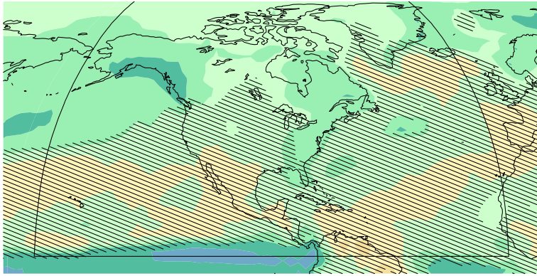
RCP2.6, 2046-2065 vs. 1986-2005
