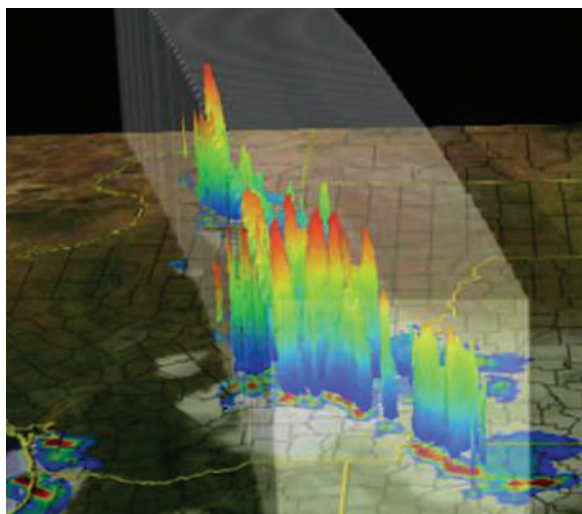
Figure 19. A snapshot of the worldwide inventory of thunderstorms from NASA's Tropical Rainfall Measuring Mission shows storms over Texas on April 30, 2004. The image shows raindrops or larger ice particles that have been carried aloft by strong rising air currents in the storms. Blue, green, and red correspond to low, moderate, and high heights, respectively. (Image courtesy NASA Goddard Space Flight Center.)
