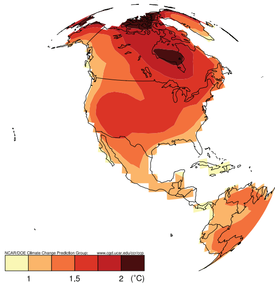
Figure 6. U.S. Temperature and Precipitation Changes by 2030. This figure shows how U.S. temperatures and precipitation would change by 2030 under IPCC emissions scenario A1B, which would increase the atmospheric concentration of greenhouse gases to about 700 parts per million by 2100 (this is roughly double the pre-industrial level). The changes are shown as the difference between two 20-year averages (2020-2040 minus 1980-1999). These results are based on simulations from nine different climate models from the IPCC AR4 multi-model ensemble. The simulations were created on supercomputers at research centers in France, Japan, Russia, and the United States. (Adapted by Lawrence Buja and Julie Arblaster from Tebaldi et al. 2006: Climatic Change, Going to the Extremes; An intercomparison of model-simulated historical and future changes in extreme events , Climatic Change , 79:185-211.)
