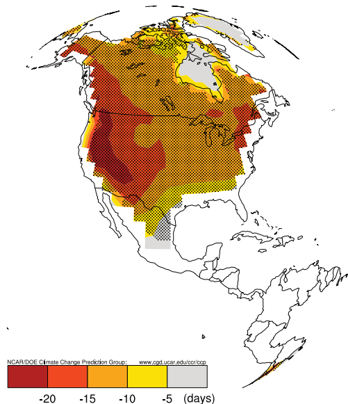
IPCC A1B Frost Days 2030-1990
