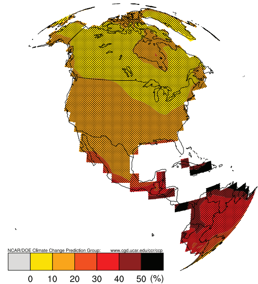
IPCC A1B Warm Nights 2030-1990
