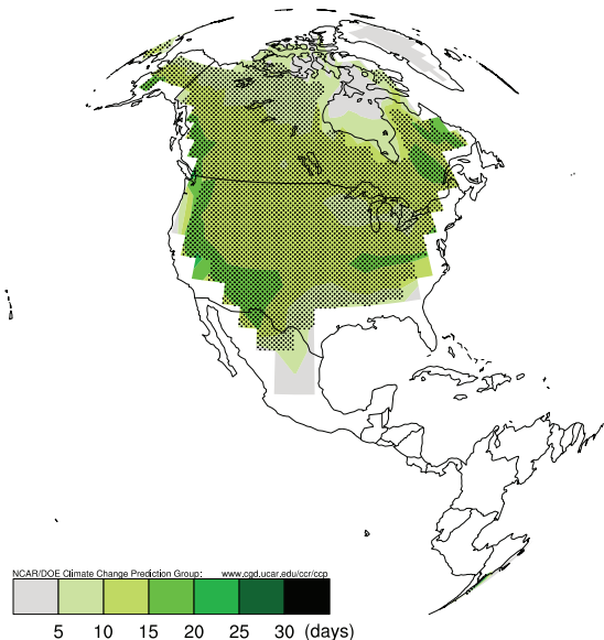
IPCC A1B Growing Season 2030-1990
