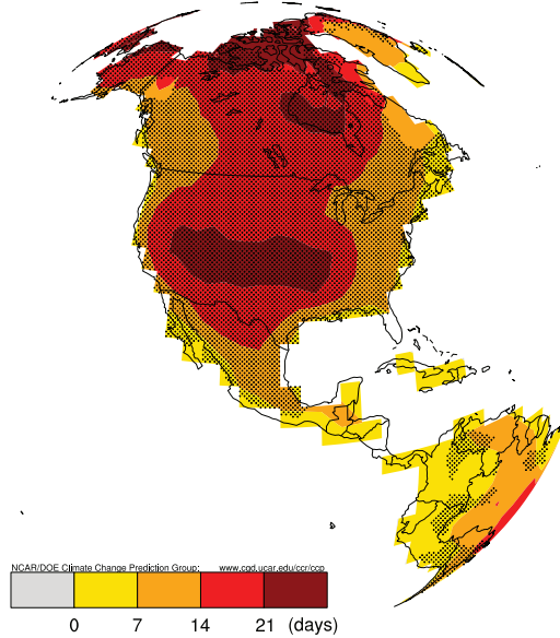
IPCC A1B Heat Waves 2030-1990
