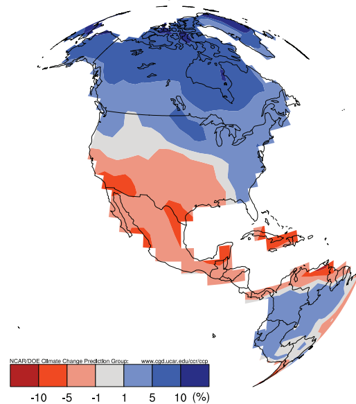
Figure 6. U.S. Temperature and Precipitation Changes by 2030. This figure shows how U.S. temperatures and precipitation would change by 2030 under IPCC emissions scenario A1B, which would increase the atmospheric concentration of greenhouse gases to about 700 parts per million by 2100 (this is roughly double the pre-industrial level). The changes are shown as the difference between two 20-year averages (2020-2040 minus 1980-1999). These results are based on simulations from nine different climate models from the IPCC AR4 multi-model ensemble. The simulations were created on supercomputers at research centers in France, Japan, Russia, and the United States. (Adapted by Lawrence Buja and Julie Arblaster from Tebaldi et al. 2006: Climatic Change, Going to the Extremes; An intercomparison of model-simulated historical and future changes in extreme events , Climatic Change , 79:185-211.)
