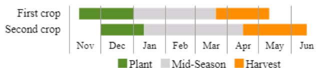
Argentina Soybean
