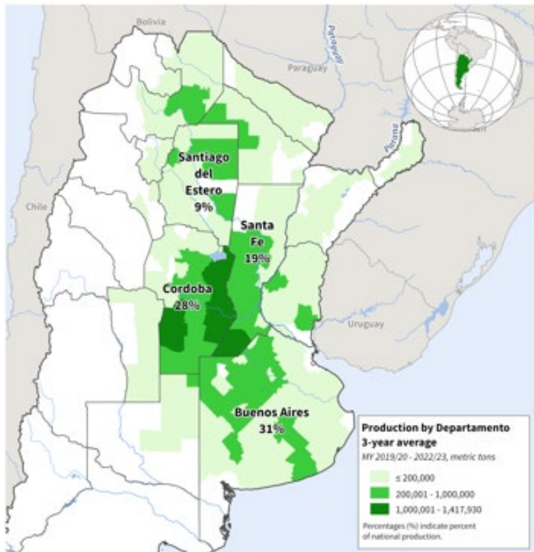
Argentina Soybean
