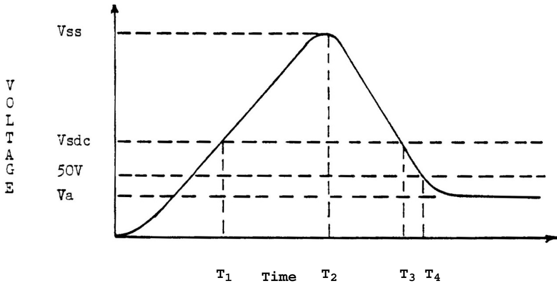
FIGURE 2: ARRESTER BREAKDOWN NOMENCLATURE
